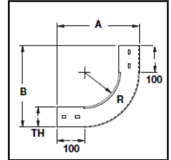
Inside Riser
