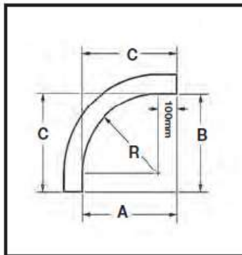
Outside Riser
