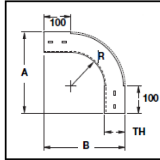
Outside Riser
