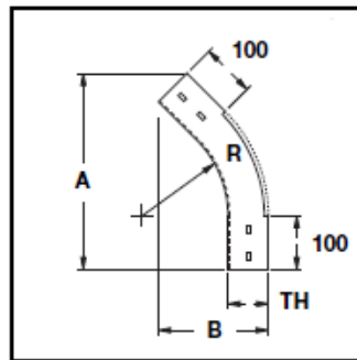
Outside Riser
