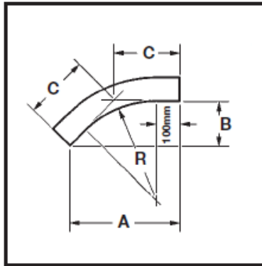
Outside Riser
